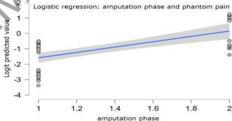
Figure 2. Graphical representation of the applied logistic regression, which in this case was used to examine the association between the amputation phase and the occurrence of phantom limb pain. The blue line represents the logistic regression prediction, while the shaded area corresponds to the 95% confidence interval
